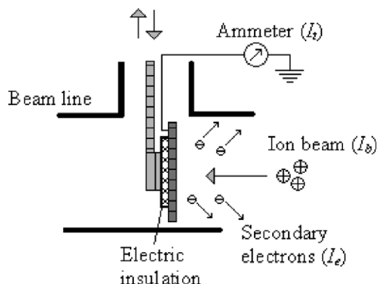
Fig. 2. Schematic of the beam-stop device in the HCII showing the interaction of the ion beam with copper plate: I_t , current measured by the ammeter; I_b , ion beam current; I_e , secondary electron current.
